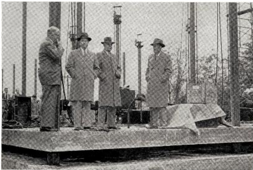
GOING UP on the first lift slab being used in the construction of the new television-radio building for WFBC-AM-TV Greenville, S. C., are (l to r) Bevo Whitmore, WFBC-AM-TV general manager; Wilson Wearn, WFBC-AM-TV assistant to the president; R. A. Jolley, WFBC-AM-TV president, and Sam Hooks, Daniel Co. project engineer. Daniel Co. is general contractor for the project; engineers are Lyles, Bissett, Carlisle & Wolff of Columbia, S. C. Provisions for transmission of network color programs coincidental with occupancy of the building have been announced by the station.
